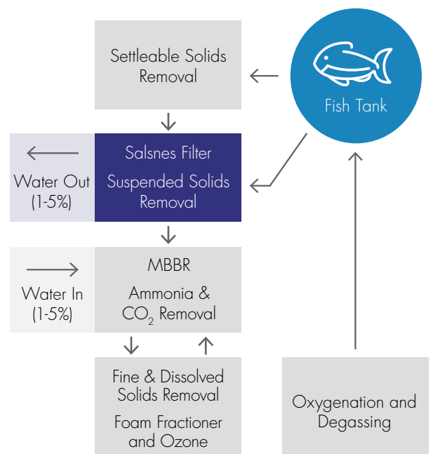
The process stream at Lensvik Hatchery
